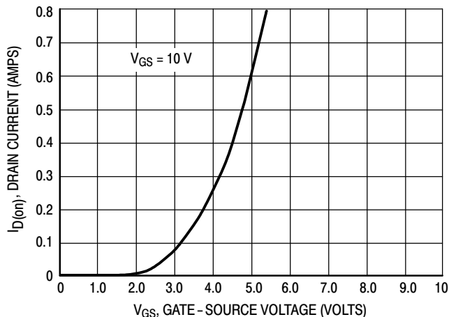
Figure 5. Transfer Characteristic
