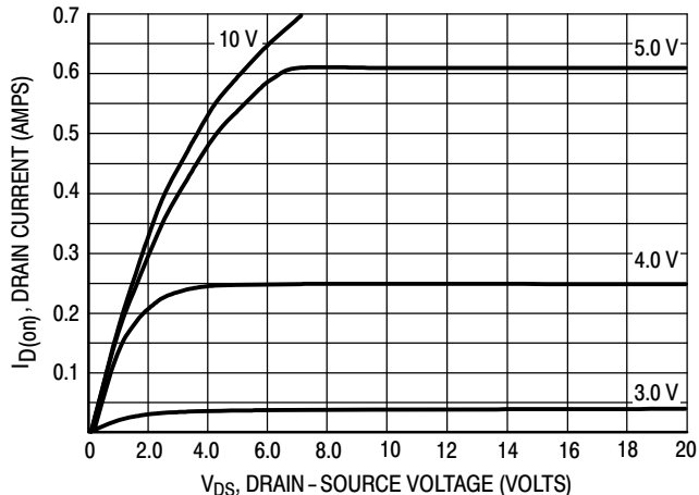
Figure 6. Output Characteristic
